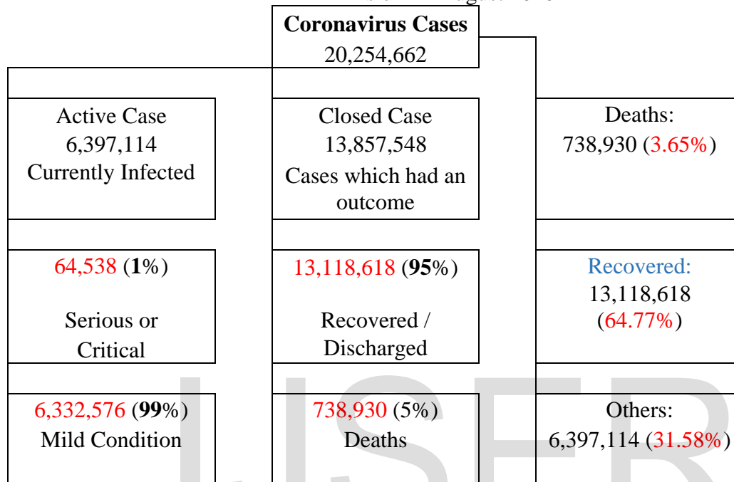
Fig 03: Situation of Global Coronavirus Cases As on 11 August 2020
